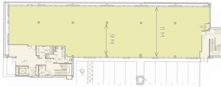
GROUND FLOOR
